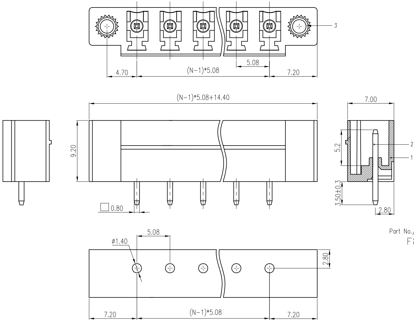
PCB LAYOUT
